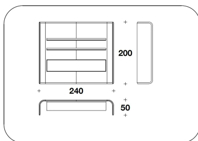
MDB (25P) - MDB (25E) MATT VENEERED : CABINET 240x50x200H.cm 94 1/3x19 3/4x78 2/3H. "
