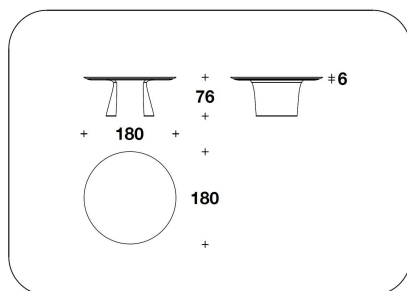
BTV (32EE) - BTV (32EP) - BTV (32EE/SCZ) ROUND : TAVOLO / TABLE Ø 180x76H. - THK.6cm Ø 71x30H. - THK.2 6/16"
