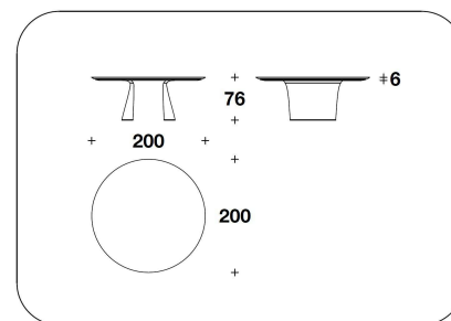
BTV (30EE) - BTV (30EP) - BTV (30EE/SCZ) ROUND : TAVOLO / TABLE Ø 200x76H. - THK.6cm Ø 78 2/3x30H. - THK.2 6/16"
