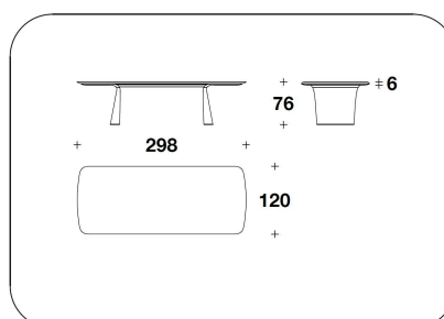
BTV (29ME) - BTV (29MP) - BTV (29ME/SCZ) RECTANGULAR MARBLE : TAVOLO / TABLE 298x120x76H. - THK.6cm 117 1/3x47 1/3x30H. - THK.2 6/16"
