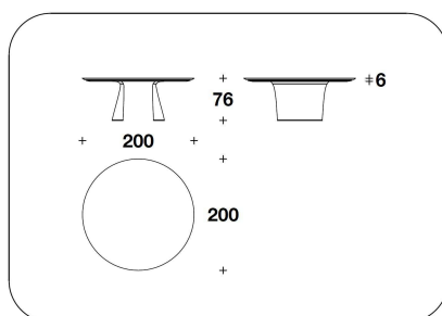
BTV (30ME) - BTV (30MP) - BTV (30ME/SCZ) ROUND MARBLE : TAVOLO / TABLE Ø 200x76H. - THK.6cm Ø 78 2/3x30H. - THK.2 6/16"
