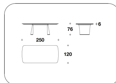
BTV (31ME) - BTV (31MP) - BTV (31ME/SCZ) RECTANGULAR MARBLE : TAVOLO / TABLE 250x120x76H. - THK.6cm 98 1/3x47 1/3x30H. - THK.2 6/16"
