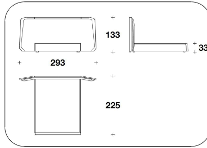
PST (LE1E) VENEERED BASE : LETTO PER MATERASSO / BED FOR MATTRESS 165x200 - 293x225x133H. - H.B.33cm 65x78 2/3 - 115 1/3x88 2/3x52 1/3H. - H.B.13"
