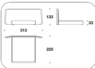
PST (LE2E) VENEERED BASE : LETTO PER MATERASSO / BED FOR MATTRESS 185x200 - 313x225x133H. - H.B.33 cm 73x78 2/3 - 123 1/3x88 2/3x52 1/3H. - H.B.13 "
