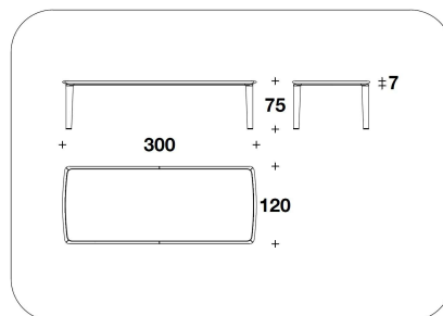
BTV (16EE) - BTV (16EP) TAVOLO / TABLE 300x120x75H. - THK.7cm 118x47 1/3x29 2/3H. - THK.2 3/4"
