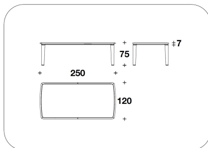
BTV (15EE) - BTV (15EP) TAVOLO / TABLE 250x120x75H. - THK.7cm 98 1/3x47 1/3x29 2/3H. - THK.2 3/4"
