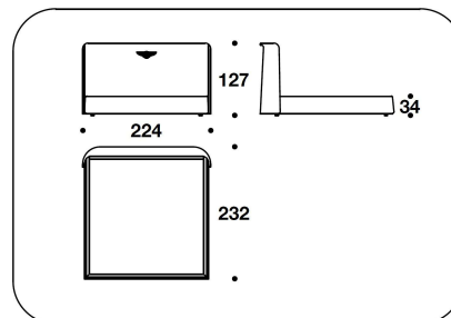
LBM (LE7) LETTO PER MATERASSO / BED FOR MATTRESS 200x200 - 224x232x127H. - H.B.34cm 78 2/3x78 2/3 - 88 1/3x91 1/3x50H. - H.B.13 2/4"
