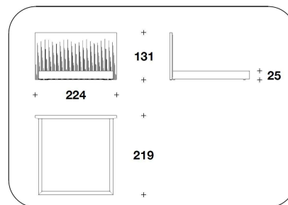
ANG (LE2) LETTA PER MATERASSO / BED FOR MATTRESS 185x200 - 224x219x131H. - H.B.25cm 73x78 2/3 - 88 1/3x86 1/3x51 2/3H. - H.B.9 3/4"
