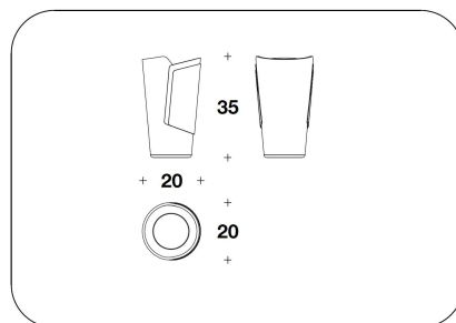
VAB (13) VASO / VASE Ø 20x35H. cm Ø 7 3/4x13 3/4H. "
