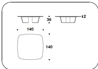
CTB (07M) MARBLE : COFFEE TABLE 140x140x36H.cm 55x55x14 1/4H."
