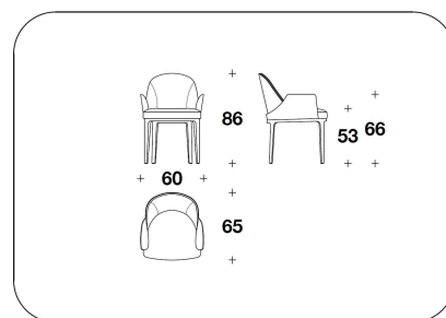
SDB (13B) SEDIA CON BRACCIOLI / CHAIR WITH ARMRESTS 60x65x86H. - H.A.66 - H.S.53cm 23 2/3x25 2/3x34H. - H.A.26 - H.S.21"
