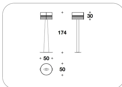
LMB (22) LAMPADA DA TERRA / FLOOR LAMP Ø 50x174H.cm Ø 19 3/4x68 2/3H."
