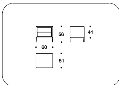
BCM (1P) TAVOLO NOTTE / BEDSIDE TABLE 60x51x56H.cm 23 2/3x20x22H."
