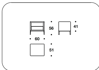
BCM (1R) BURR WALNUT : TAVOLO NOTTE / BEDSIDE TABLE 60x51x56H.cm 23 2/3x20x22H."
